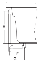
DRAIN/OVERFLOW
