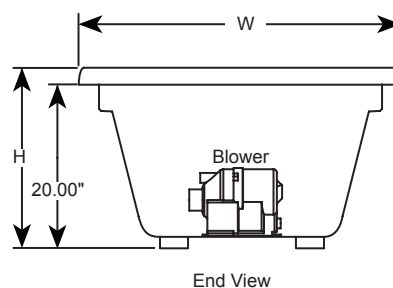
End View
