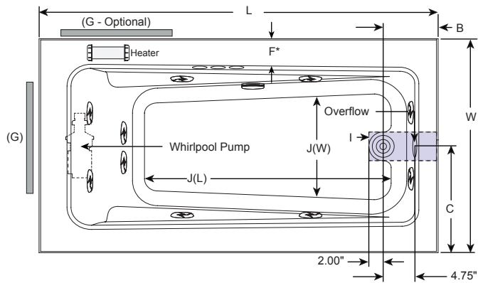
Installed Right-Hand Orientation
