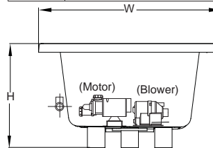
End View
