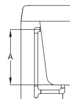
Drain/Overflow
